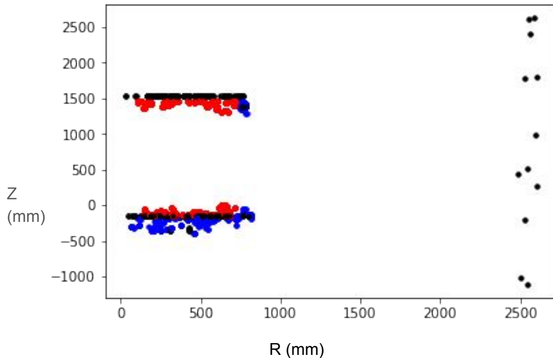
Th-232 Decay chain events originating from PMT windows. Primary Events (Black), Inside the TPC (Red), In LXe Skin (Blue)
