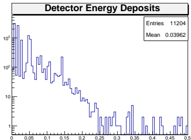
Figure 2: Energy Deposits without removing Muon tagged events
