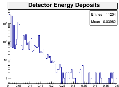
Figure 4: Energy Deposits without removing Muon tagged events
