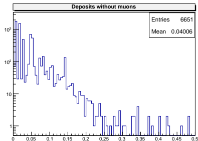
Figure 3: Energy Deposits after removing muons
