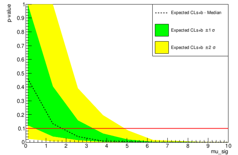
Toy = 1000
