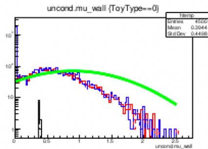
Sigma = 0.8
