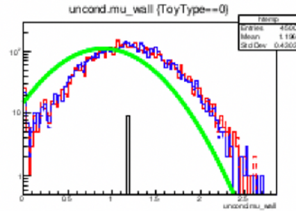
Sigma = 0.5
