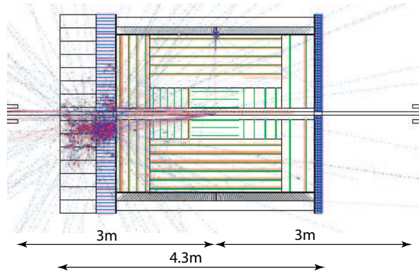
FIGURE 2. Side view of the GEANT detector implementation as part of the ELECTRA simulation and reconstruction package [6]. A deep-inelastic scattering event resulting from a LEPTO simulation is overlaid with Q^2 = 361 \text{ GeV}^2 and x = 0.45 .
