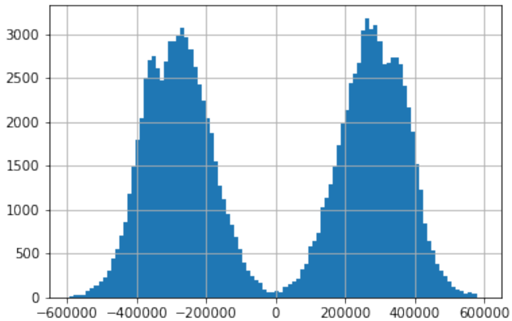
7:Z Position
