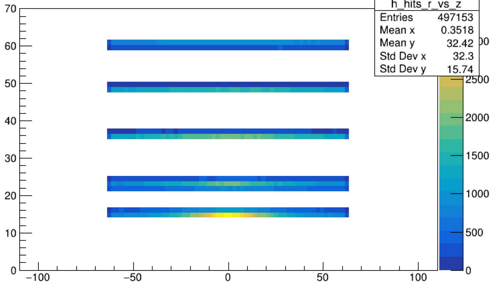
h_hits_r_vs_z
