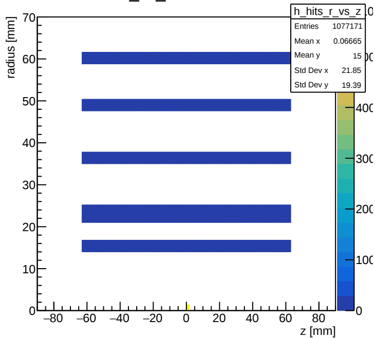
R_vs_z Process 4
