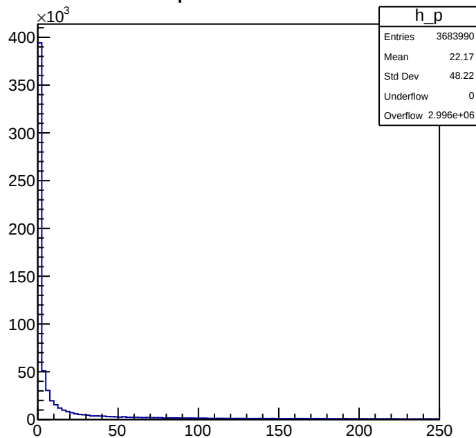
p Process 2
