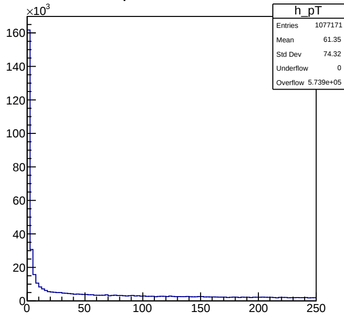
pT Process 4
