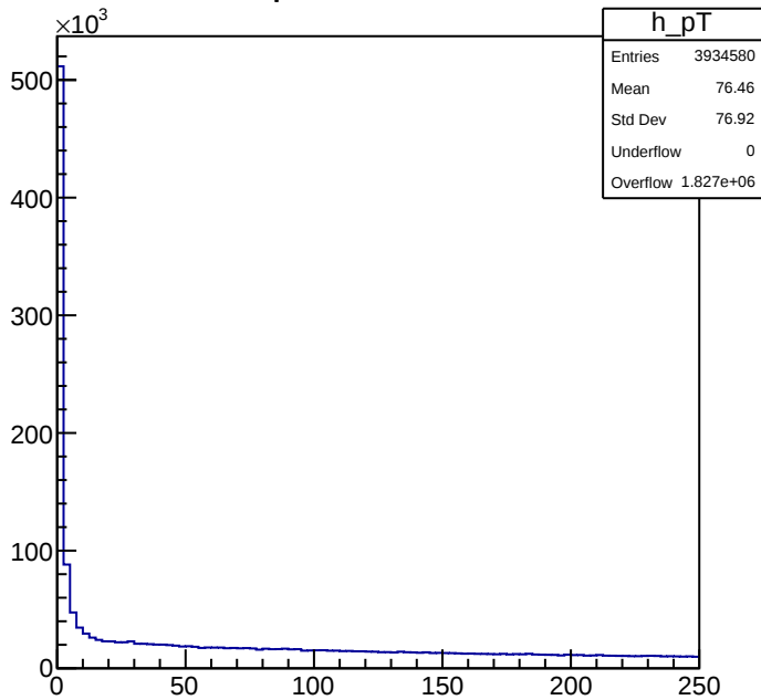
pT Process 1
