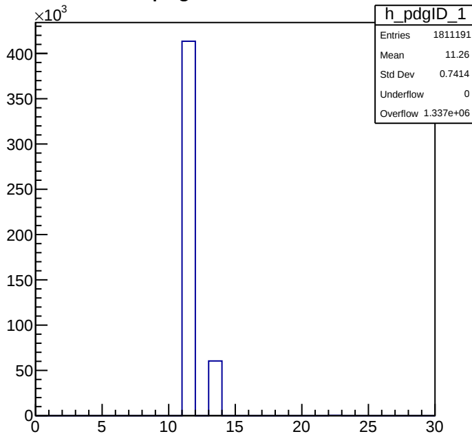
pdgID Process 1
