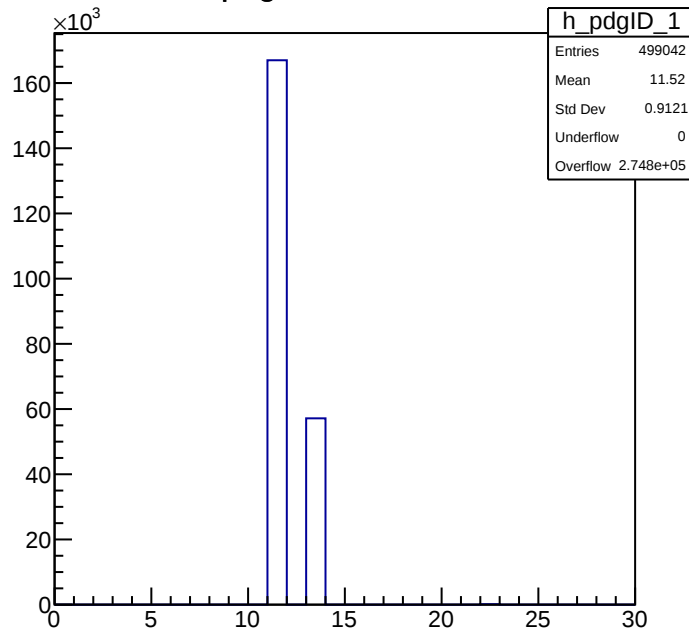
pdgID Process 4
