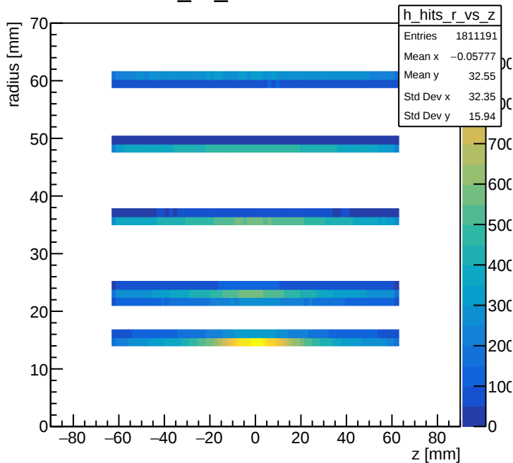
R_vs_Z Process 1
