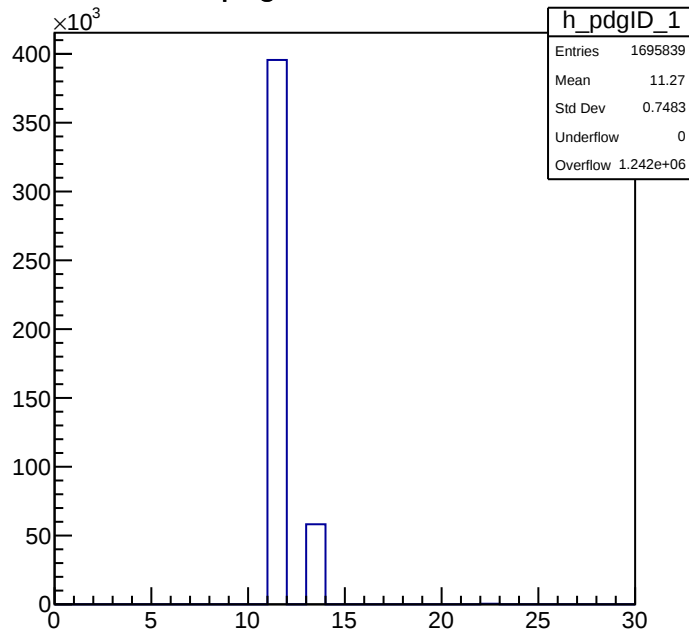
pdgID Process 2
