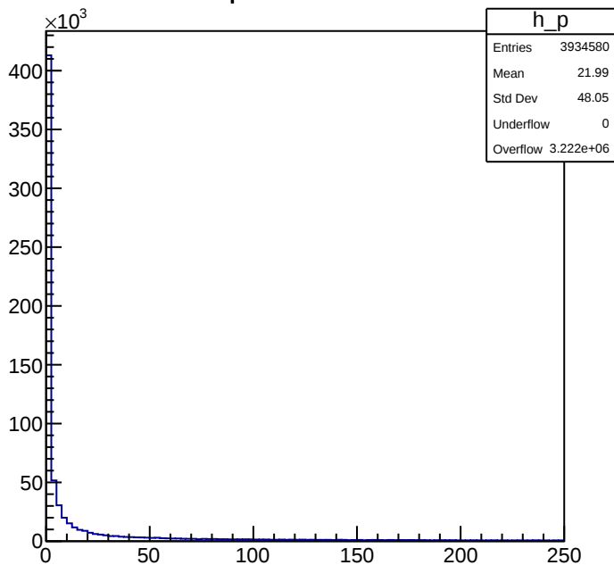
p Process 1
