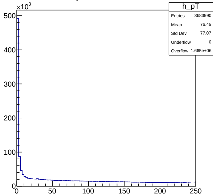
pT Process 2
