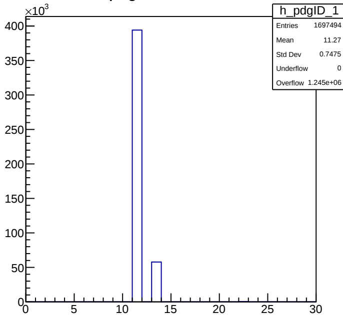
pdgID Process 3
