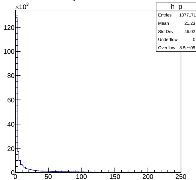
p Process 4
