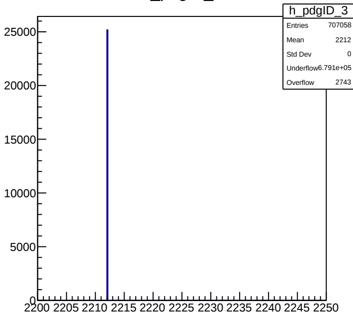
h_pdgID_3
