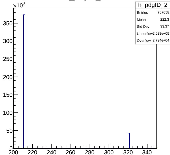
h_pdgID_2
