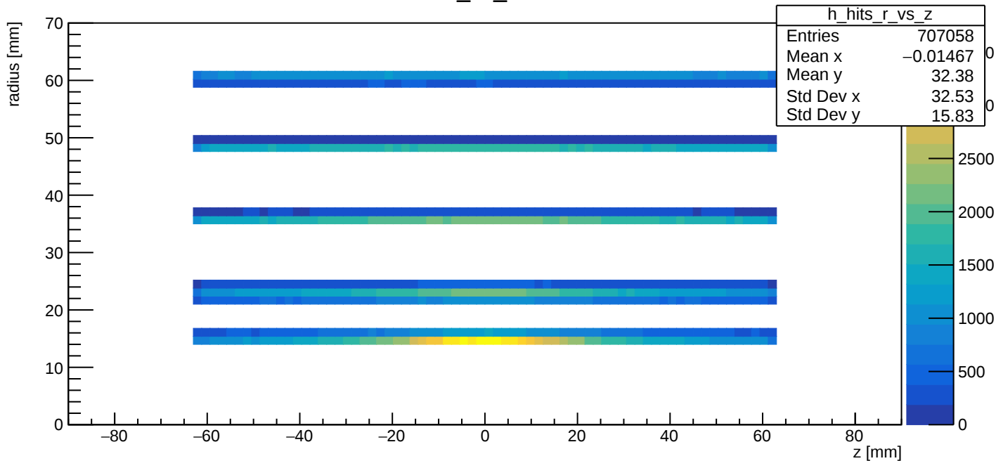
r_vs_Z
