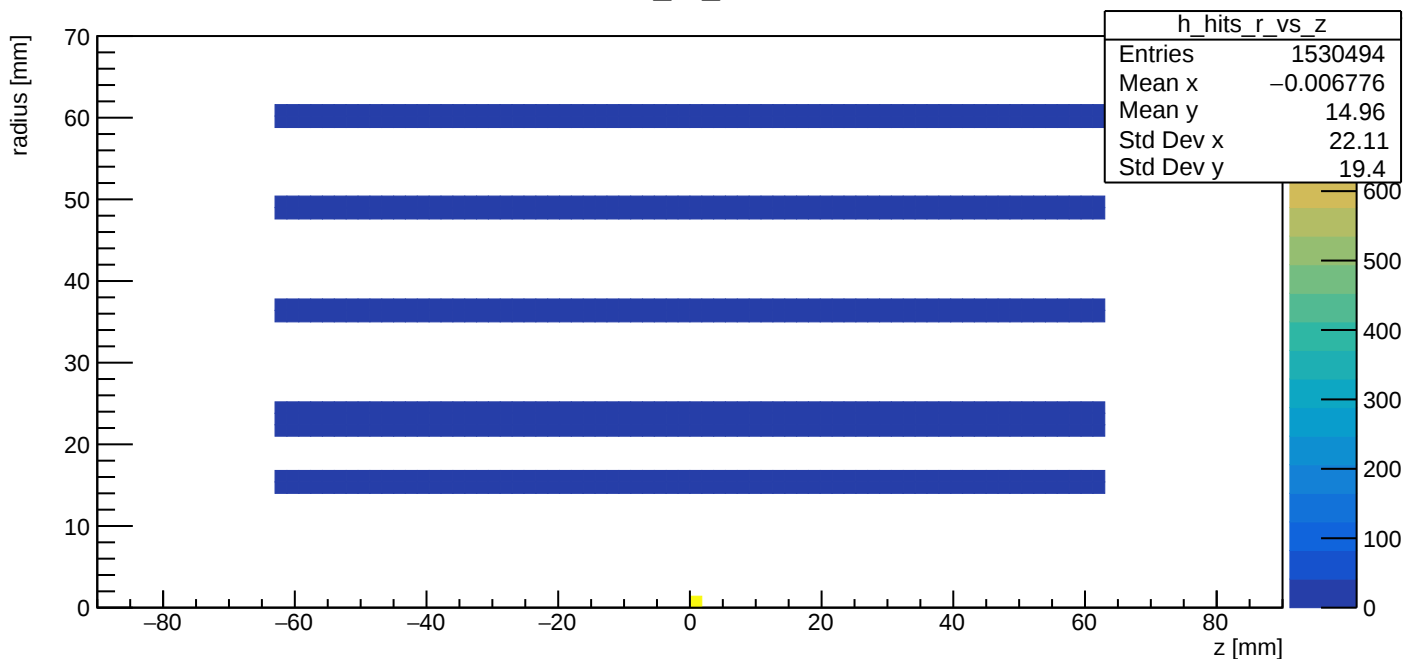
r_vs_Z
