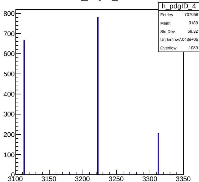
h_pdgID_4
