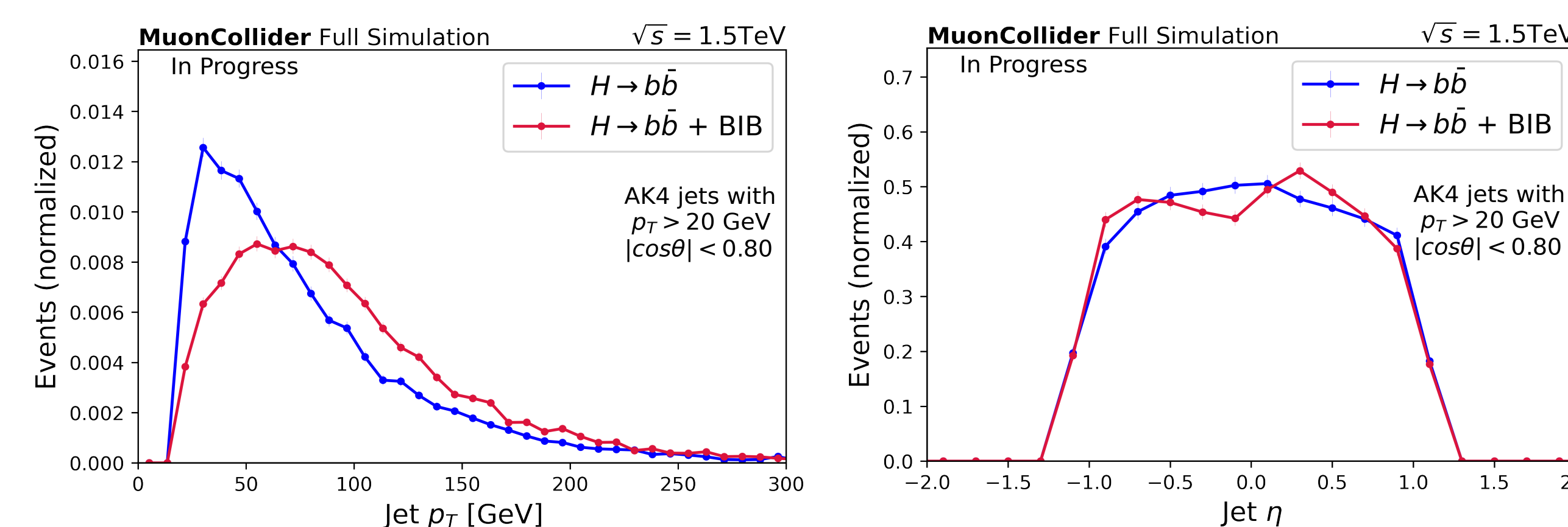
Figure 6: Jet p_T (left) and \eta (right) with (red) and without (blue) BIB presence. The overlay of BIB hits result in reconstructed jets with higher p_T and forward \eta .
