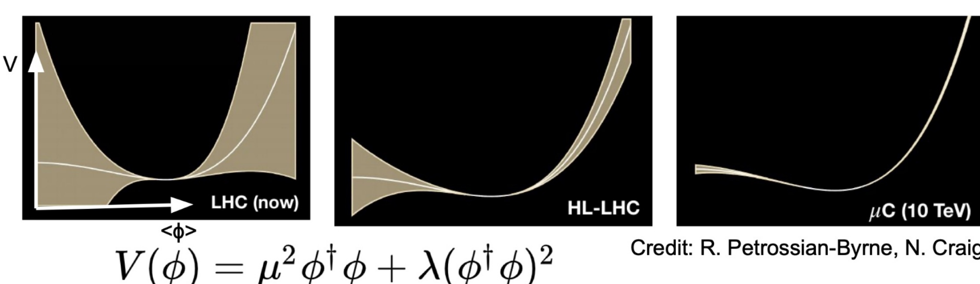
Figure 2: MC can probe Higgs potential to higher precision
