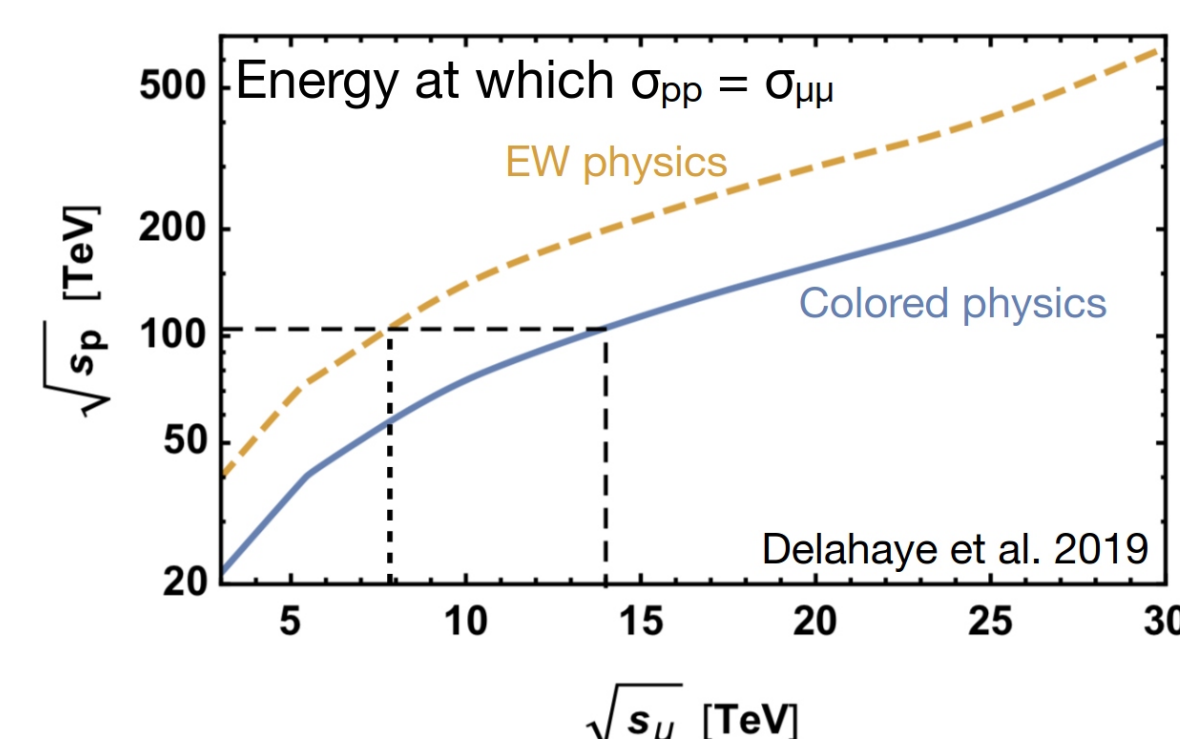
Figure 1: Physics reach of muon collider at 14TeV ~ pp collider at 100 TeV
