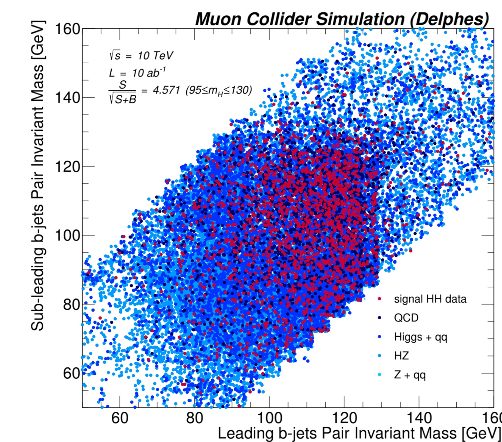
Figure 8: 4 channel event distribution of both signal and backgrounds channels in Leading and Sub-leading b -Jet Pairs Invariant Mass Plane for \sqrt{s} = 10 TeV data.
