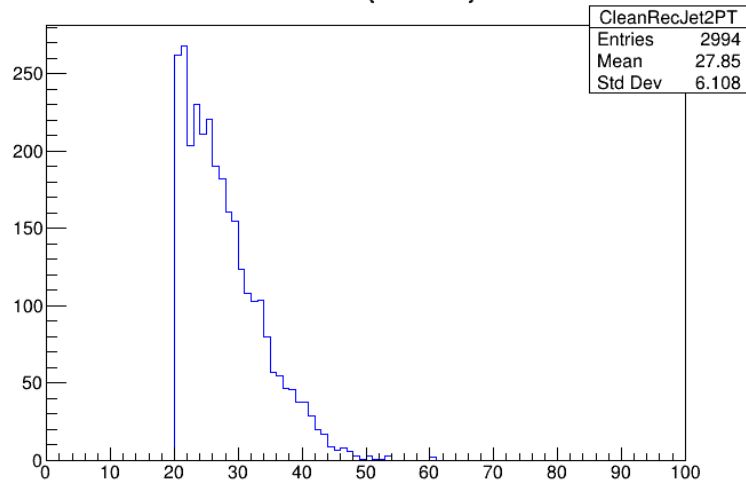
Clean PT {RecJet2}
