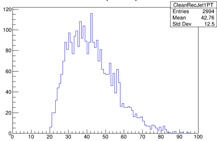
Clean PT {RecJet1}
