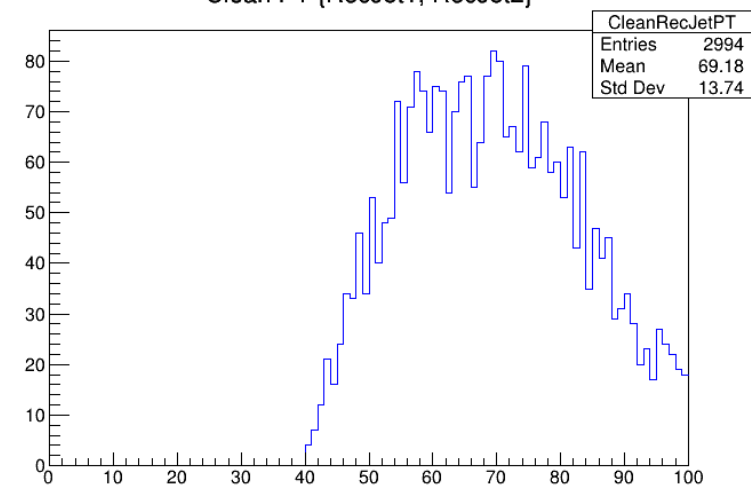
Clean PT {RecJet1, RecJet2}
