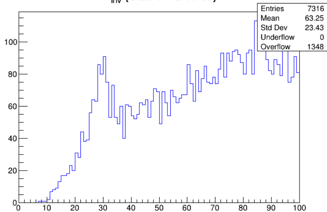
M_{\text{inv}} {Stable Particles}
