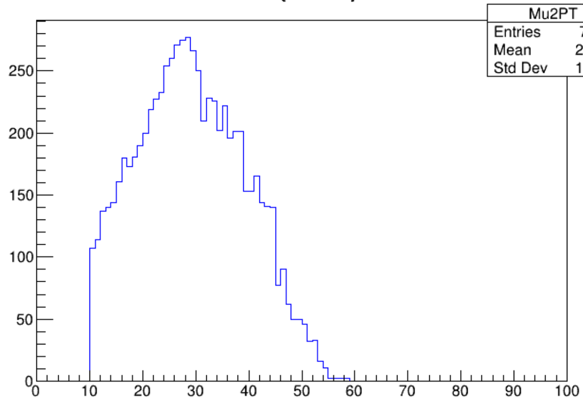
PT {Muon2}
