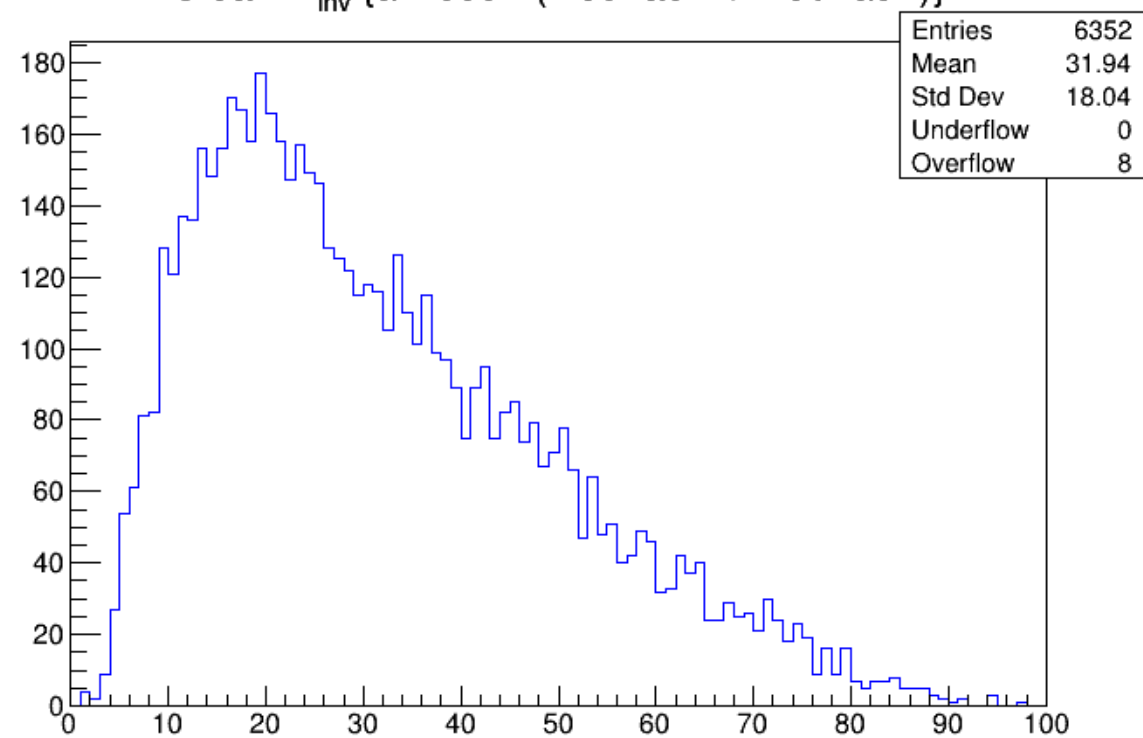
Clean M_{\text{inv}} {a Boson (RecTau1 + RecTau2)}
