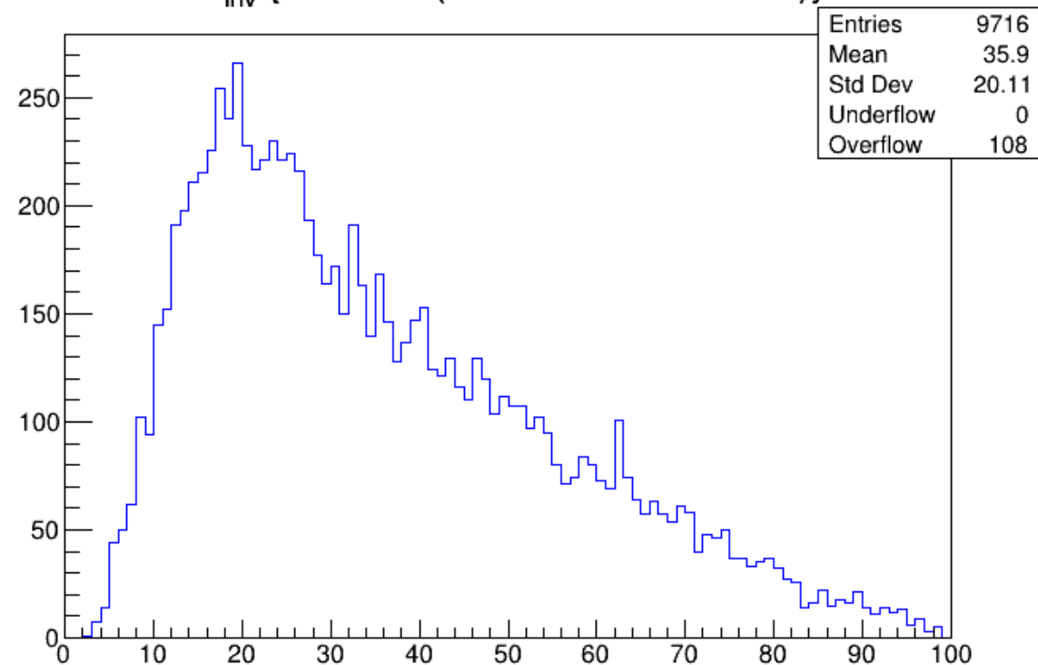
M_{inv} {Z Boson (RecTau1 + RecTau2)}
