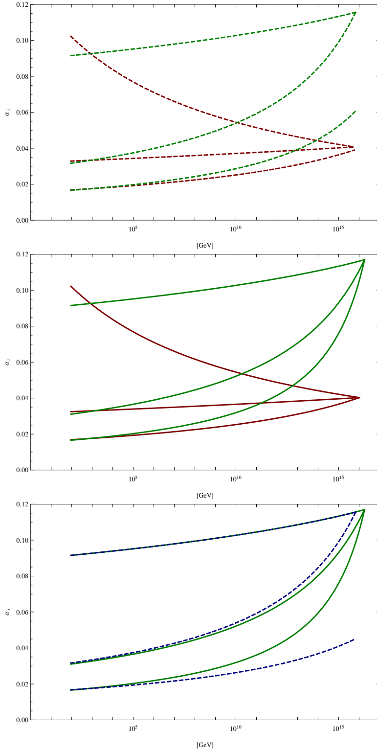
FIG. 3: Running of the gauge couplings is compared for \mathcal{F}\text{-SU}(5)_0 (dash red) Vs. \mathcal{F}\text{-SU}(5)_{\text{II}} (dash green), \text{SU}(5)_0 (solid red) Vs. \text{SU}(5)_I (solid green), and \text{SU}(5)_I (solid green) Vs. \mathcal{F}\text{-SU}(5)_I (dash blue). The upper line of each set depicts \alpha_3 . The apparent mismatch of couplings departing M_Z is strictly a visual artifact of choosing to absorb thresholds and the second loop from the outset, as elaborated in the text.
