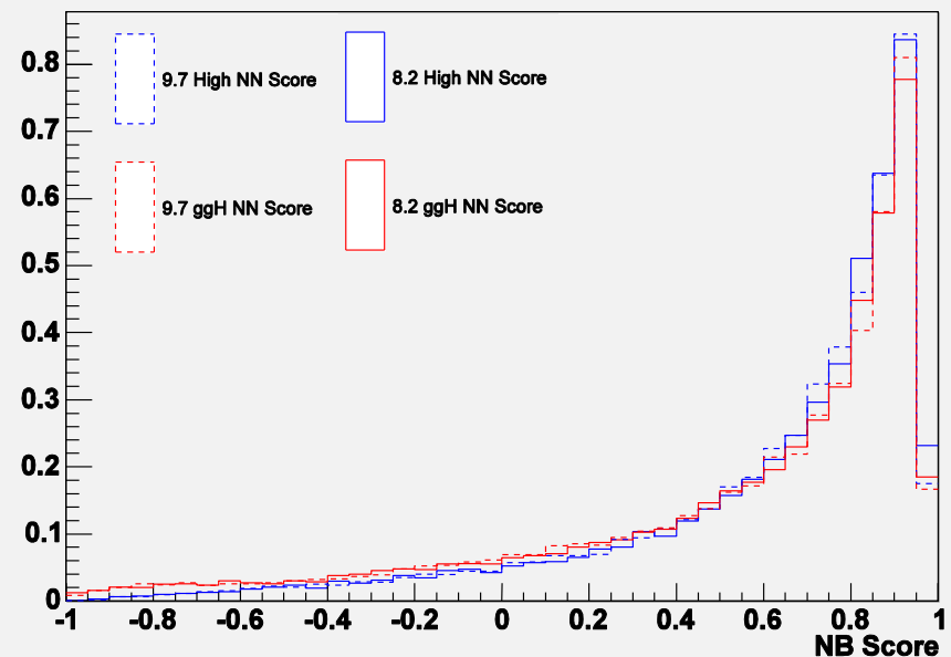
Neural Net Scores for ggH Events
