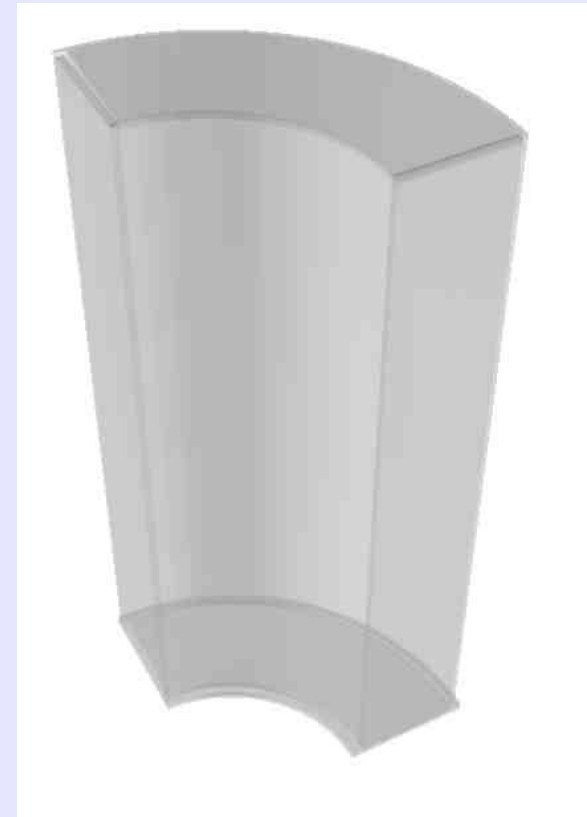
Geant4
