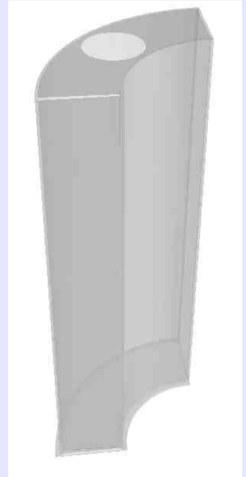
Geant4
