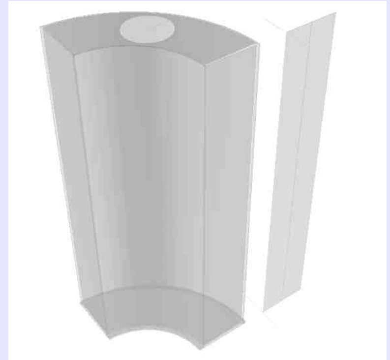
Same Design in Geant4
